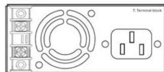
Terminal Block
