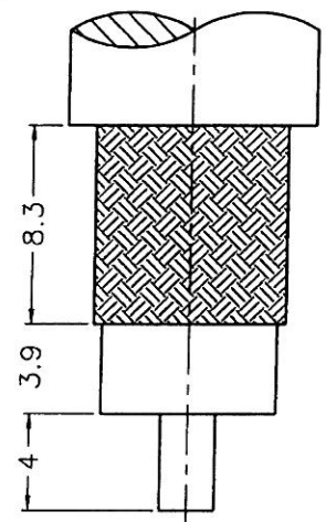
RECOMMENDED CABLE STRIPPING DIM'S (建議剝線尺寸)
