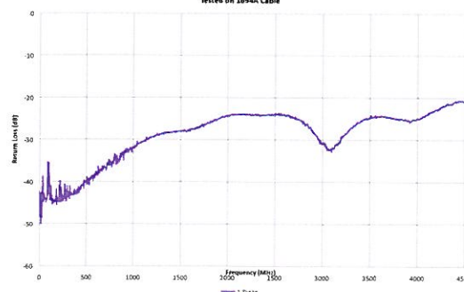
Connector RL Performance Tested on 1694A Cable
